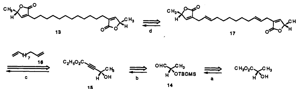
Scheme 1. Retrosynthesis and Synthesis of (+)-Ancepsenolide a
